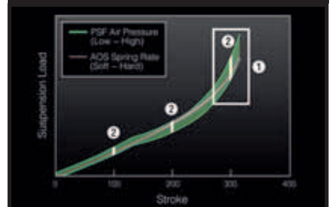
Air/Spring behaviour
